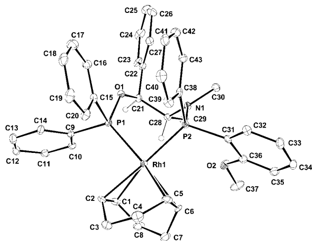
Figure 2. ORTEP representation of the [(COD)Rh(AMPP 4b )]BF 4 complex 9 . For clarity, only one molecule is shown. Selected bond lengths [Å], angles, and dihedral angles [°] for one of the two molecules: P1–O1 1.619 (3), P2–N1 1.666 (3), P1–Rh1 2.2773 (10), P2–Rh1 2.3229 (10), Rh1–HC28 2.641; P1–Rh2–P2 88.54 (4); O1–P1–P2–N1 21.83 (15), P1–O1–C21–C22 177.96 (23), P1–O1–C28–C29 139.87 (45), phenyl planes C15–C20 and C38–C43 14.00 (21), phenyl–anisyl planes C9–C14 and C31–C36 31.43 (21). The thermal ellipsoids are drawn at 50% probability. The H atoms are not shown for clarity, except for those on the C21 and C28 carbon atoms.
