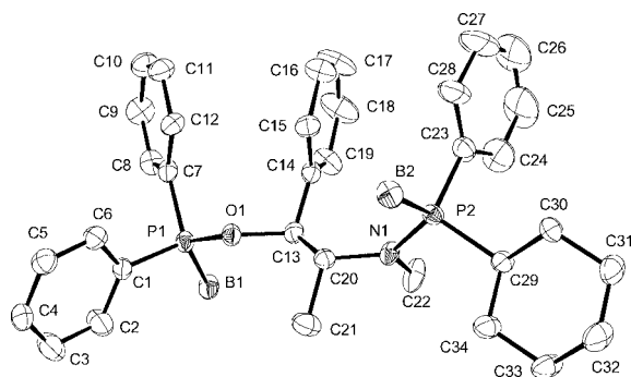
Figure 1. ORTEP representation of AMPP-diborane complex 7j . For clarity, only one independent molecule is shown. Selected bond lengths [Å], angles [°], and dihedral angles [°] for one of the two molecules: P1–B1 1.904 (2), P2–B2 1.915 (3), P2–N1 1.6697 (17), P1–O1 1.6111 (14); C20–N1–P2 121.83 (13), C22–N1–P2 121.21 (14); C22–N1–C20 116.58 (16), B2–P2–N1–C22 173.99 (18), B2–P2–C23–C28 3.58 (24), O1–C13–C20–N1 172.87 (15), B2–P2–C29–C30 58.63 (18), B2–P2–C29–C34 65.82 (17). The thermal ellipsoids are drawn at 50% probability. The H atoms are not shown for clarity.
