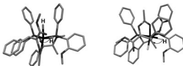
Figure 3. Computer model for the [Rh(AMPP 4b)H 2 (substrate 1)] intermediates 10a-re (left) and 10b-re (right) with the C=C branched on the west side, showing plausible hydride nucleophilic attacks on the re face of the substrate, both resulting in the same observed (S) product 2.
